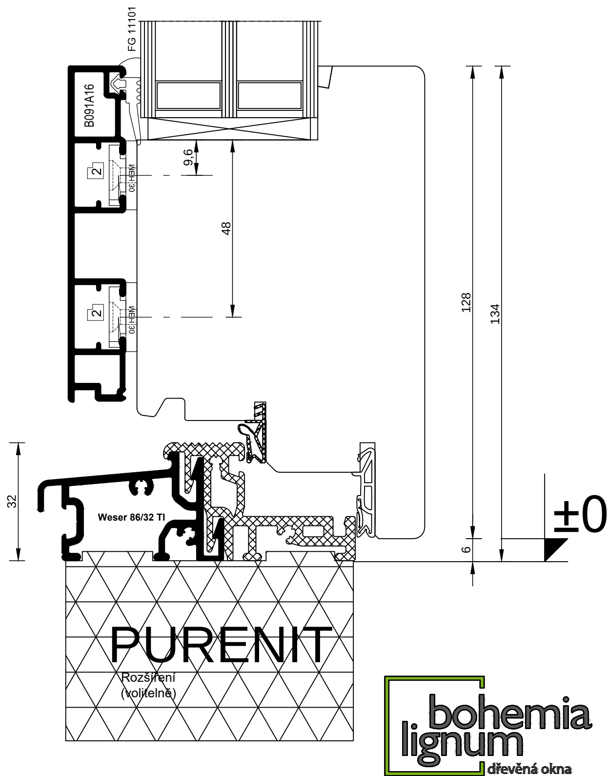
BLA300/80S_Glass_48mm/005.1
