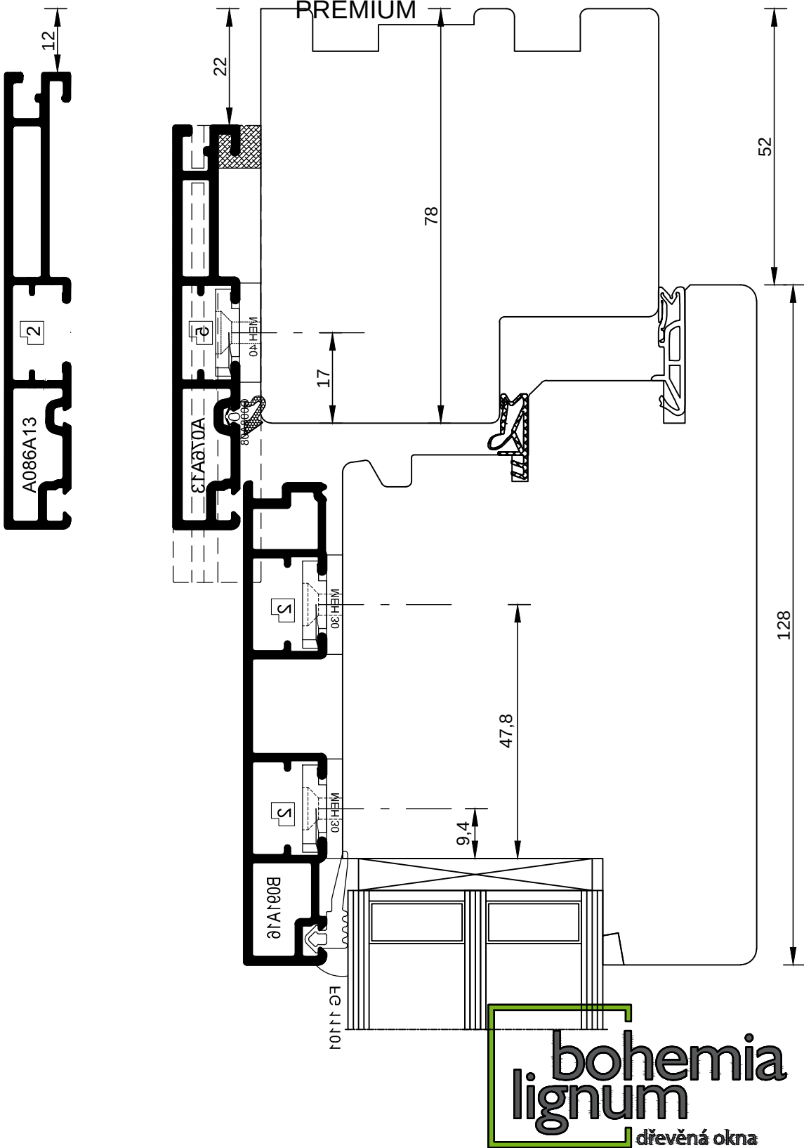
BLA300/80S_Glass_48mm/005.2
