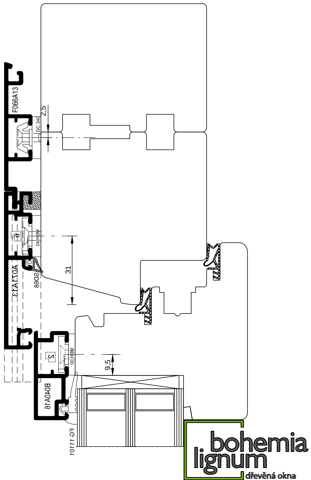
BLA300/80S_Glass_48mm/008.1 20180802.1
